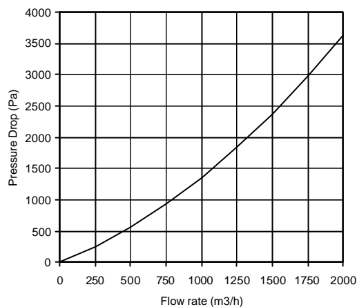
Typical Pressure Drop of VENTSORB ® 120R - CENTAUR ® HSV
